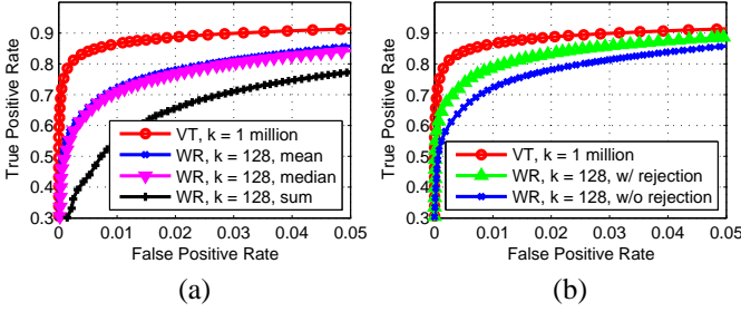
Fig. 3. (a) ROCs for Vocabulary Tree (VT) and Word Residuals (WRs) with three aggregation methods. (b) ROCs for VT and WRs with and without outlier rejection.
