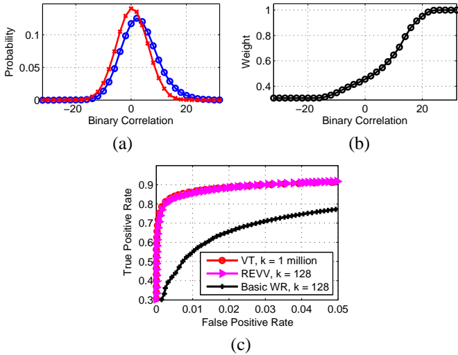
Fig. 5. (a) Distributions of binary correlation per visual word, for matching (blue o) and non-matching (red x) image pairs. (b) Weights for different binary correlation values. (c) ROCs for VT, REVV, and basic WR scheme.
