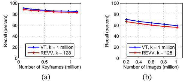
Fig. 6. Recall for (a) Stanford YouTube and (b) Stanford MVS Data Sets.
