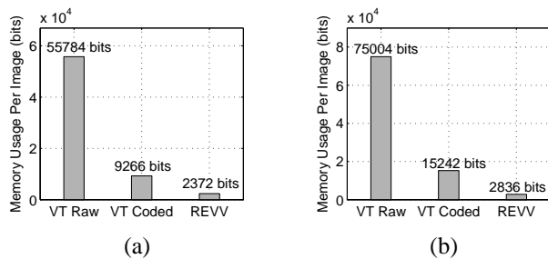
Fig. 7. Memory usage per database image for (a) Stanford YouTube and (b) Stanford MVS Data Sets.
