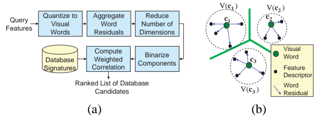
Fig. 2. (a) Overview of how feature descriptors for a query image are converted into a REVV signature and compared against database REVV signatures. (b) Visual words, feature descriptors, and sets of word residuals.
