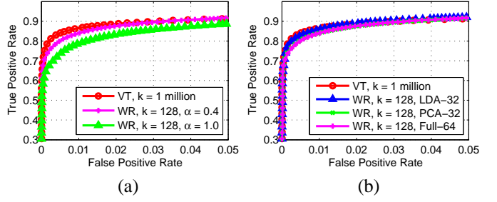
Fig. 4. (a) ROCs for VT and WRs with and without power law. (b) ROCs for VT and WRs with no transform (full 64 dimensions per word), with PCA (32 dimensions per word), and with LDA (32 dimensions per word).
